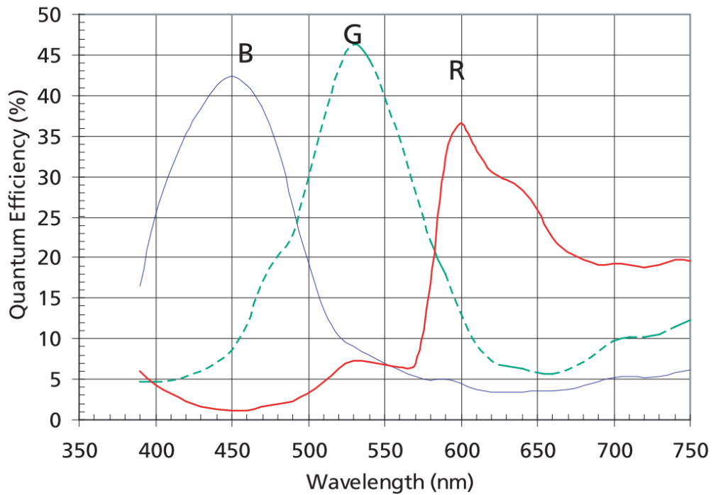
Figure 19: MT9P001 Color
