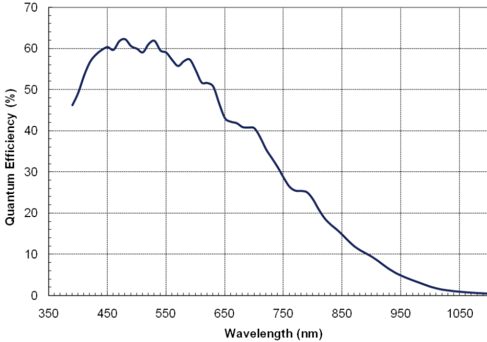
Figure 18: MT9P031 BW
